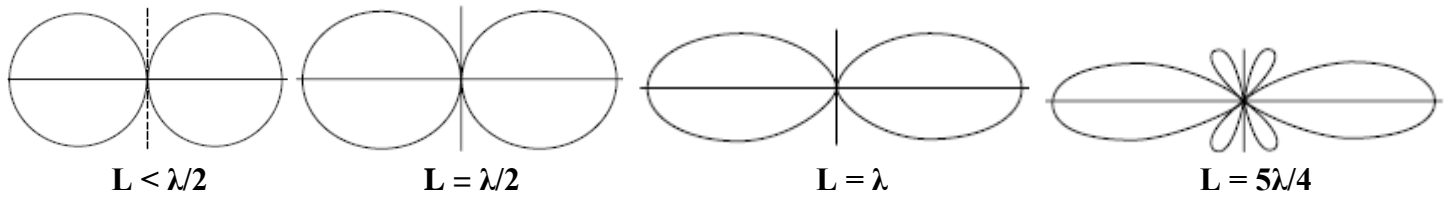
Antenna Patterns for various Dipole lengths
